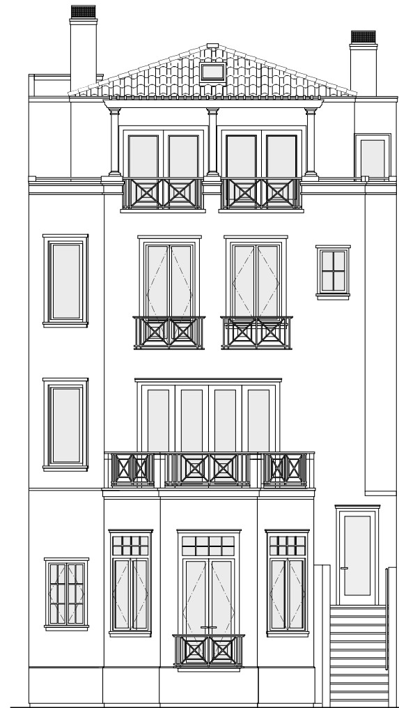
REAR YARD ELEVATION
